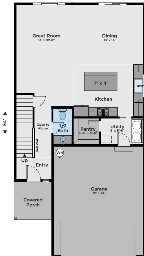
First Floor ◀ 28' ▶
